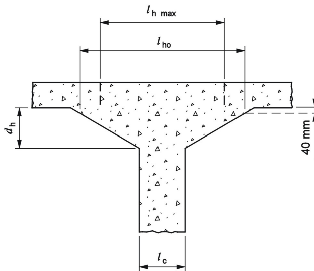
Figure 6.8 - Types of column head
