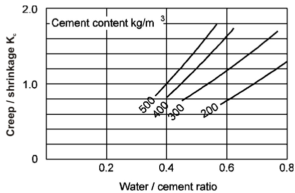
Figure 3.3 - Coefficient K_c (Creep and shrinkage)
